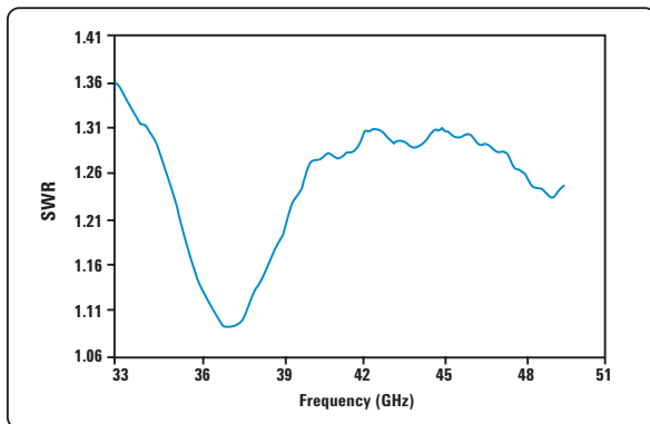
Typical SWR, 33 GHz to 50 GHz ( 25\text{ }^{\circ}\text{C}\pm 10\text{ }^{\circ}\text{C} ) for N8486AQ power sensor
