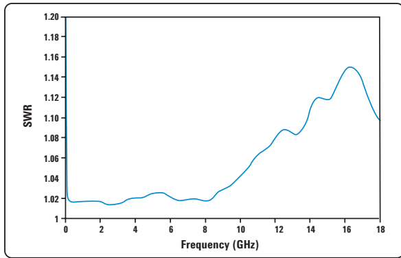
Typical SWR, 10 MHz to 18 GHz ( 25\text{ }^{\circ}\text{C}\pm 10\text{ }^{\circ}\text{C} ) for N8481A sensor
