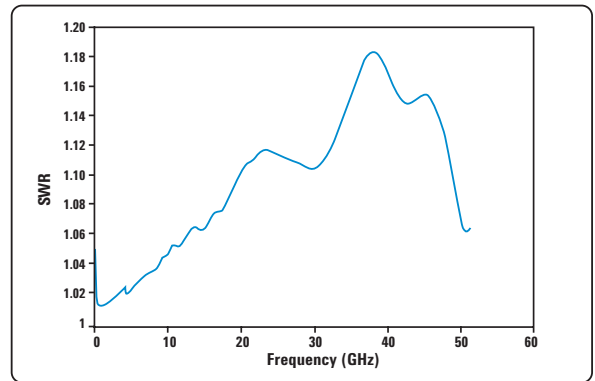
Typical SWR, 50 MHz to 50 GHz ( 25\text{ }^{\circ}\text{C}\pm 10\text{ }^{\circ}\text{C} ) for N8487A power sensor
