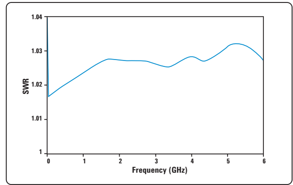
Typical SWR, 100 kHz to 6 GHz ( 25\text{ }^{\circ}\text{C}\pm 10\text{ }^{\circ}\text{C} ) for N8482A sensor
