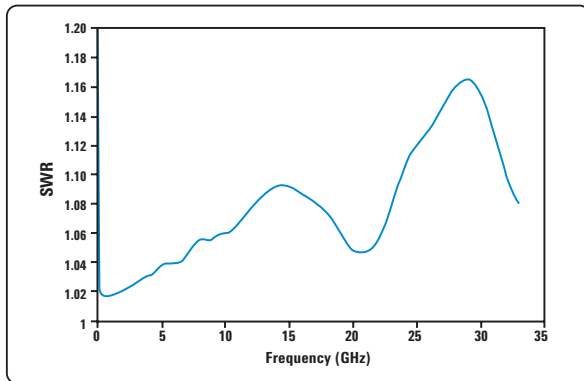
Typical SWR, 10 MHz to 26.5 GHz ( 25\text{ }^{\circ}\text{C}\pm 10\text{ }^{\circ}\text{C} ) for N8485A sensor
