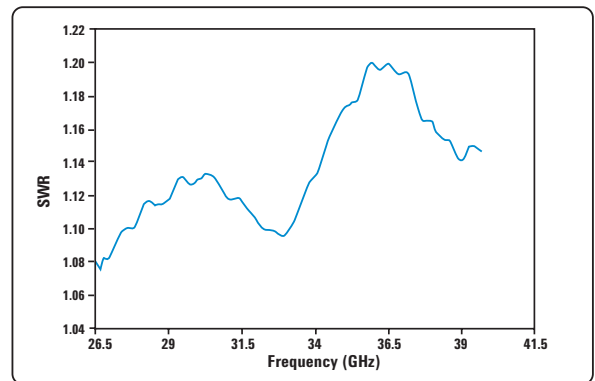
Typical SWR, 26.5 GHz to 40 GHz ( 25\text{ }^{\circ}\text{C}\pm 10\text{ }^{\circ}\text{C} ) for N8486AR power sensor
