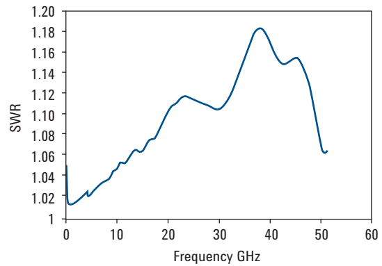
Typical SWR, 50 MHz to 50 GHz ( 25\text{ }^{\circ}\text{C} \pm 10\text{ }^{\circ}\text{C} ) for N8487A power sensor
