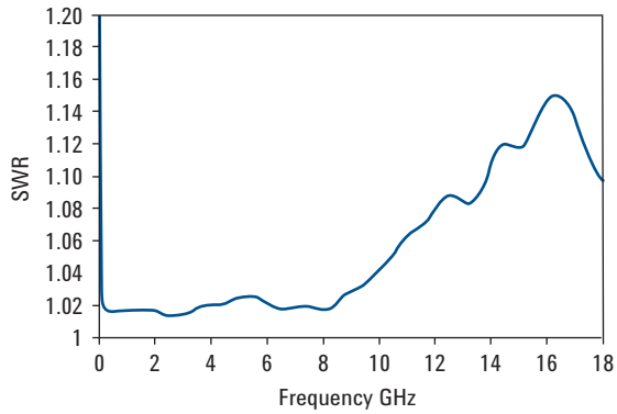
Typical SWR, 10 MHz to 18 GHz ( 25\text{ }^{\circ}\text{C} \pm 10\text{ }^{\circ}\text{C} ) for N8481A sensor
