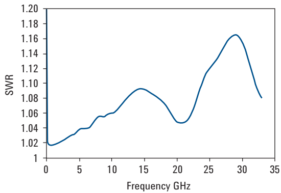
Typical SWR, 10 MHz to 26.5 GHz ( 25\text{ }^{\circ}\text{C} \pm 10\text{ }^{\circ}\text{C} ) for N8485A sensor
