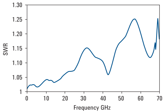
Typical SWR, 10 MHz to 70 GHz ( 25\text{ }^{\circ}\text{C} \pm 10\text{ }^{\circ}\text{C} ) for N8488A power sensor
