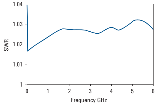
Typical SWR, 100 kHz to 6 GHz ( 25\text{ }^{\circ}\text{C} \pm 10\text{ }^{\circ}\text{C} ) for N8482A sensor
