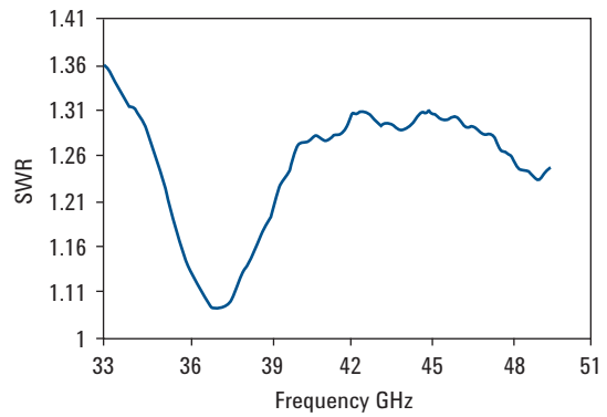
Typical SWR, 33 to 50 GHz ( 25\text{ }^{\circ}\text{C} \pm 10\text{ }^{\circ}\text{C} ) for N8486AQ power sensor
